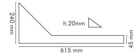
Art. 1032 - set 8 pcs./pz. Plastic fixing glass angles, low (20mm), green Angolari fermavetro in plastica, bassi (20mm), verdi
