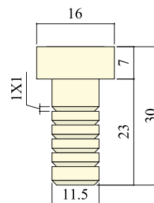
Art. 300098 Ferrule for Longoni fiber shafts, Ø 16 mm Ghiera Longoni per puntali in fibra Ø 16 mm
