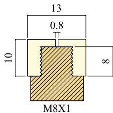
Art. 7312 FERRULE JBR POOL SLIM AND CAROM S30 GHIERA JBR POOL SLIM AND CAROM S30
