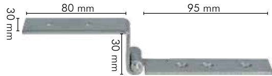
Art. 300524 Hinge for soccertables mod. Storm Cerniera per calcetto Storm
