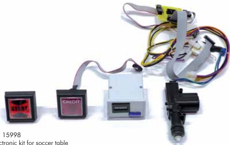
Art. 15928 Electronic kit for soccer table Kit elettronico calcetto
